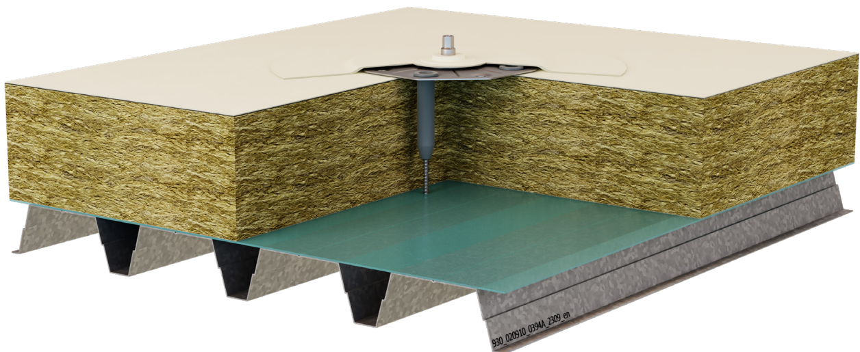
SikaRoof® Anchor Washer 140 mm fixed with Sarnafast® Fastener SBF-6.0 together with Sarnabar® Tube SBT-20. This system is used if the compression strength of the thermal insulation is slightly below 120 kPa. The maximum load per anchor needs to be reduced accordingly.
