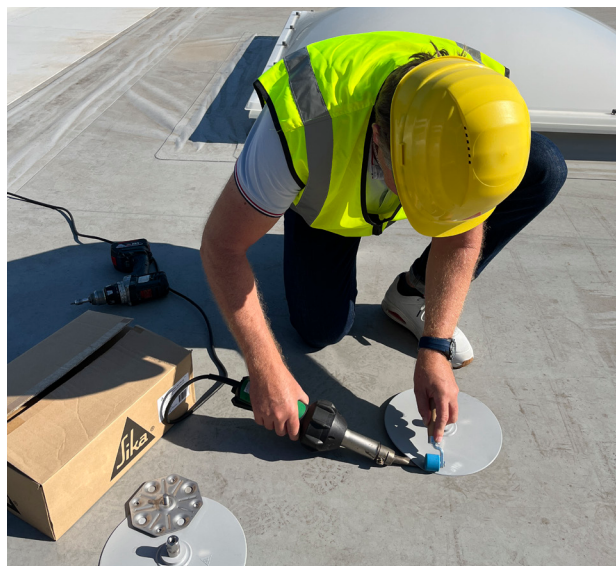
SikaRoof® Anchor 250 mm CR screwed onto the SikaRoof® Anchor Washer 140 mm and hot air welded to the roof waterproofing membrane.
